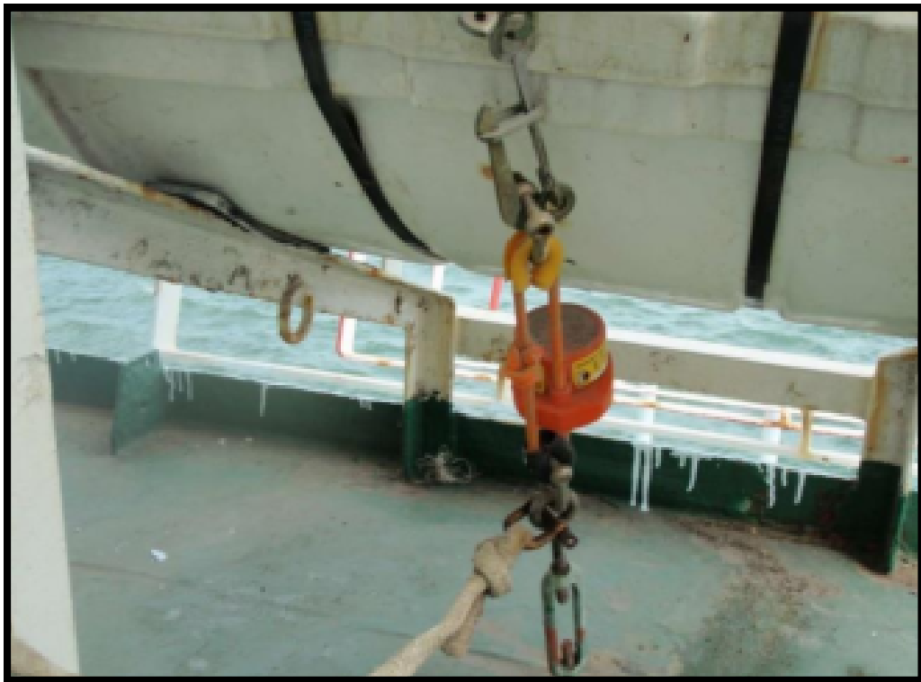
Improper connection of hydrostatic release unit (HRU)
