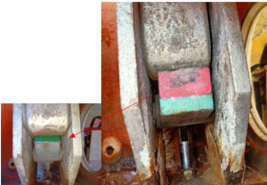
Improper reset of lifeboat release mechanism
