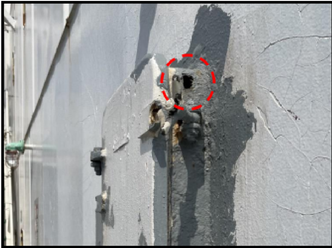
Corrosion hole on the ventilation hatch coaming
