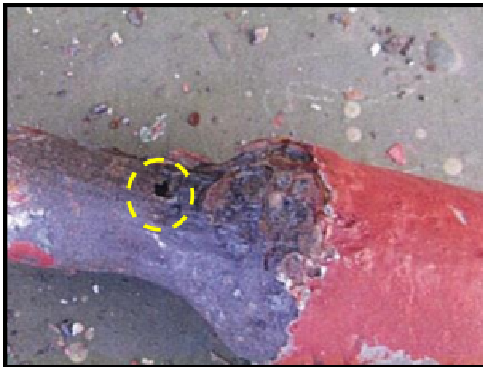
Heavy corrosion/hole on CO2 line
