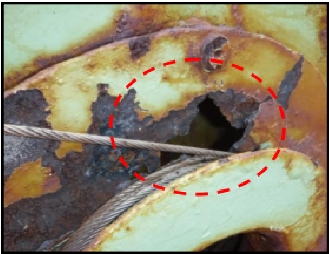
Broken wire drum
