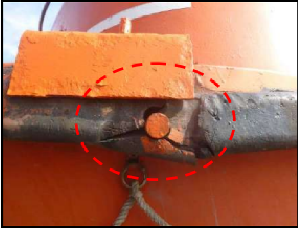
Fractured fender for life boat
