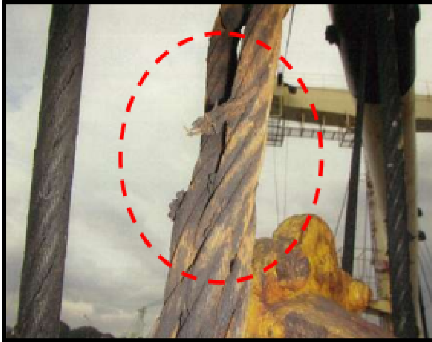
Broken wire rope for derrick
