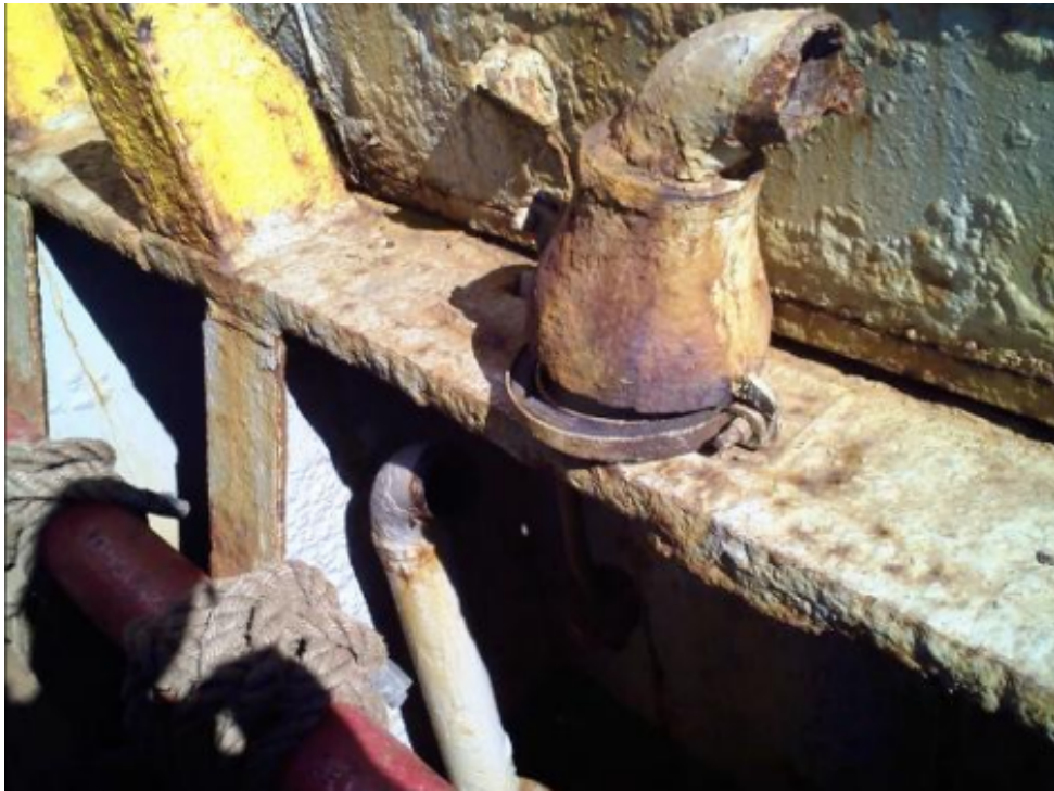
Significant corrosion and wastage on gooseneck vent.
